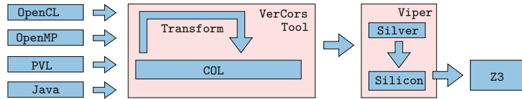
Fig. 1. The architecture of the VerCors tool.
